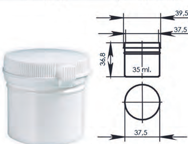
With cap KK2-2
