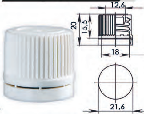
With sealing cone
