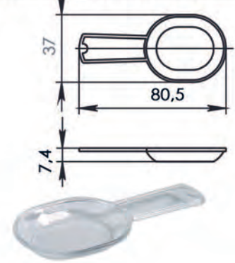
Measuring spoon type II
