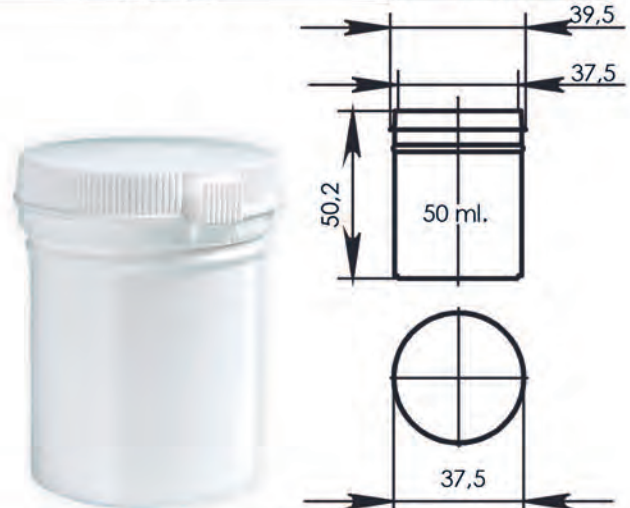
With cap KK2-2
