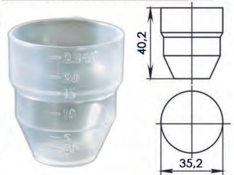
Measuring cup, 25 ml
