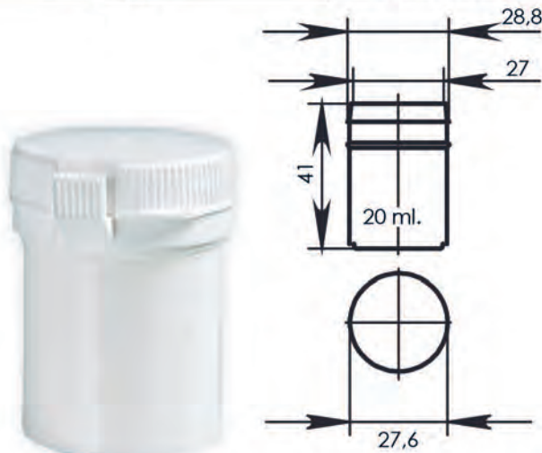
With cap KK2-1
