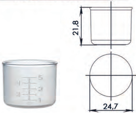
Measuring cup, 5 ml
