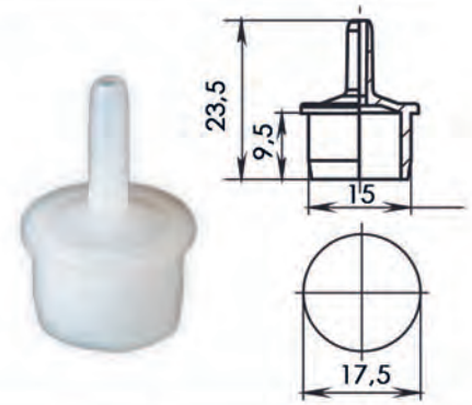
Nozzle of the container K2-55, K2-115
